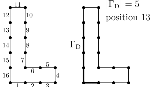
Figure 5: The L-shaped domain and enumeration of boundary segments (left). An example of a position and size of \Gamma_D (right).
