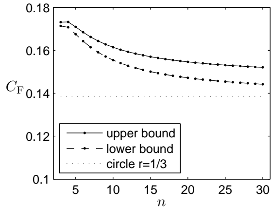
Figure 4: Values of Friedrichs' constant for n -fold regular stars.
